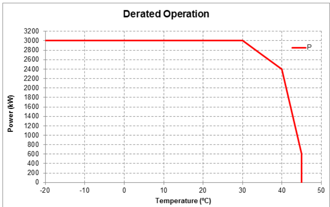
Figure 9-1: Derated operation.
